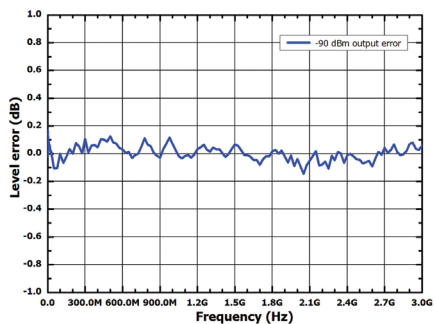
Measured at -90 dBm,level error vs.frequency
