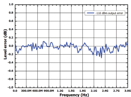
Measured at -110 dBm,level error vs.frequency
