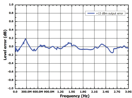
Measured at +13 dBm,level error vs.frequency
