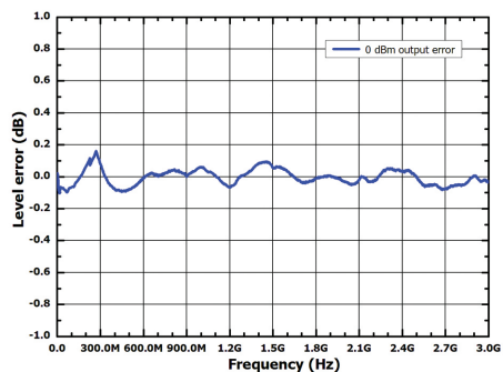
Measured at 0 dBm,level error vs.frequency
