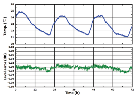
Measured level repeatability @ 1 GHz,0 dBm
