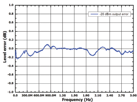
Measured at -20 dBm,level error vs.frequency
