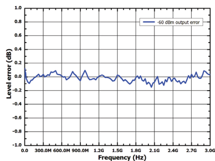
Measured at -60 dBm,level error vs.frequency
